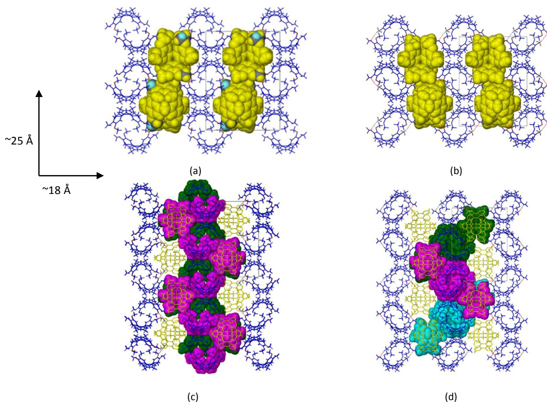
Figure 2 Packing diagrams of CTV molecules in (a) 1a and (b) 2a with 'stacked' CTV molecules shown in space-filling mode. (c) CTV molecules in 1a and (d) 2a connected by C-H...O hydrogen bonding shown in space-filling mode and the same colour. All views are down the \sim 10 Å axis.
