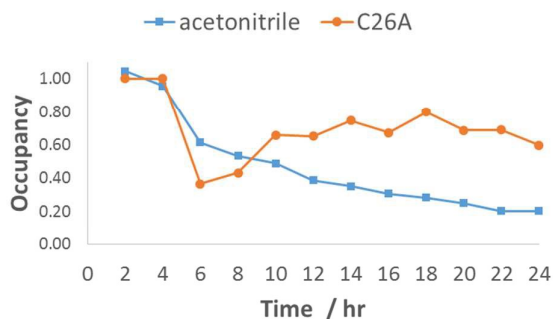
Figure 4 Occupancy of acetonitrile and C26A position after successive in situ 2 hour SCXRD data collections at 50°C. Note that acetonitrile occupancy was calculated from a SQUEEZE electron count per unit cell analysis and the C26 occupancy was refined in SHELXL-2014.
