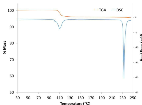
Figure 6 DSC and TGA thermograms of 1a
