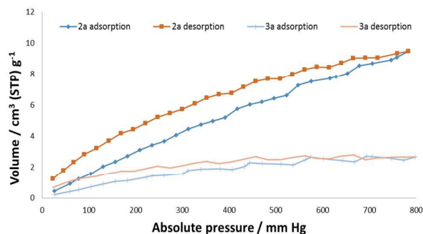
Figure 7 CO 2 sorption isotherms of 2a and 3a at 273 K.
