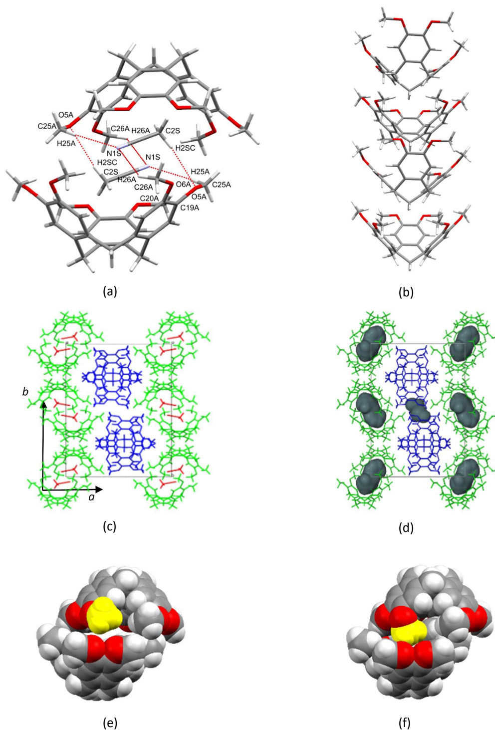
Figure 1 (a) Centrosymmetric dimer formed by ASU CTV molecule 1 (b) self-inclusion of ASU CTV molecule 2 (c) crystal packing in 1a (d) crystal packing in 2a showing isolated voids (e) dimer in 1a with the methyl group coloured in yellow corresponding to methyl group in (f) 2a that is rotated towards the interior of the cavity.
