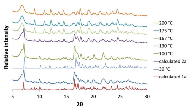
Figure 3 VT-PXRD patterns in the range 30–200 °C compared with the calculated patterns of 1a and 2a
