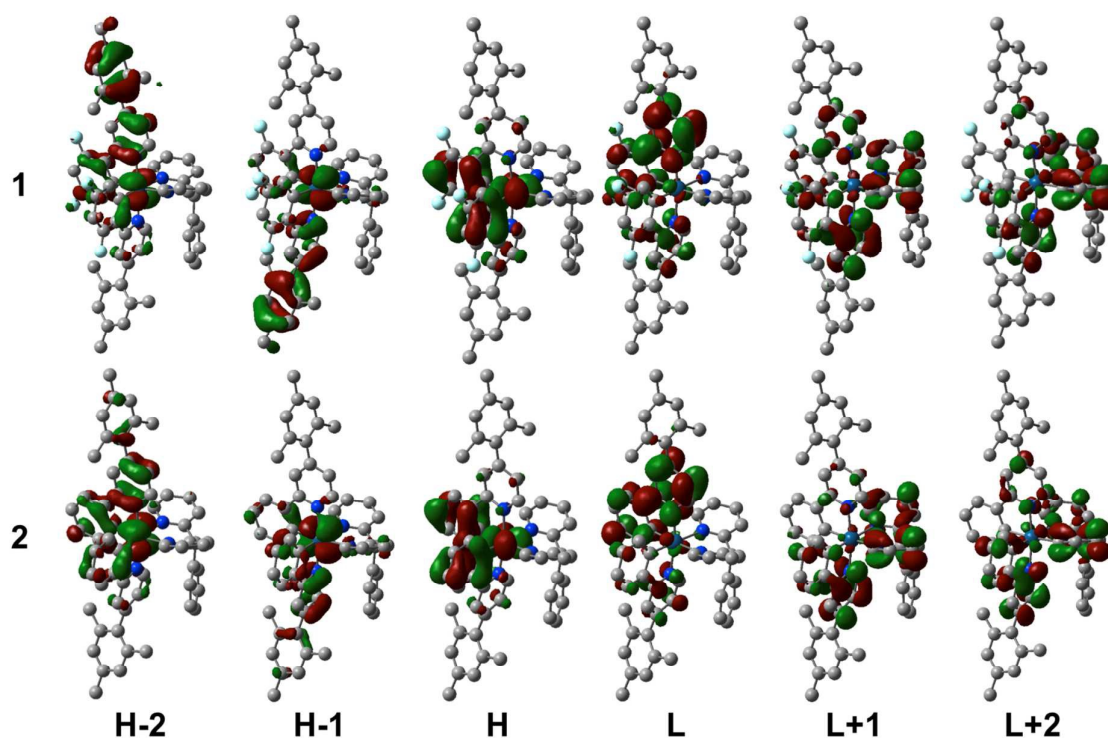
Figure 5. Representation of the six frontier orbitals of 1 (top) and 2 (bottom). A contour threshold of 0.03 au is used, and the hydrogen atoms have been omitted for clarity.
