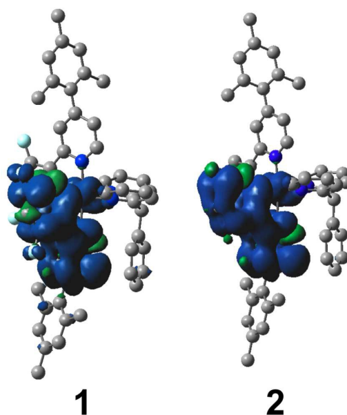
Figure 6. Representation of the spin density difference plot for 1 (left) and 2 (right). Contour threshold: 0.0008 au.
