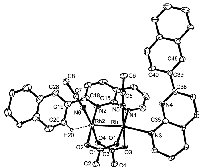
Figure 5. ORTEP diagram (30% probability thermal ellipsoids) of the cationic unit [\text{Rh}_2(\text{nplNP})(\eta^1\text{-nplNP})(\text{OAc})_2(\text{CH}_3\text{CN})_2]^{2+} in compound 7 with important atoms labeled. Hydrogen atoms, except for the agostic hydrogen, are omitted for the sake of clarity.
