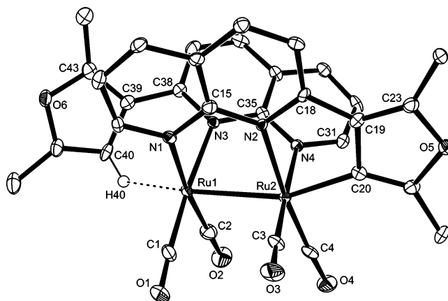
Figure 2. ORTEP diagram (50% probability thermal ellipsoids) of the cationic unit [\text{Ru}_2(\text{Me}_2\text{fuNP})(\text{C}_4\text{OMe}_2\text{-NP})(\text{CO})_4]^+ in compound 2 with important atoms labeled. Hydrogen atoms, except for the agostic hydrogen, are omitted for the sake of clarity.
