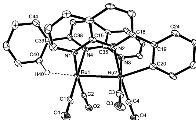
Figure 1. ORTEP diagram (50% probability thermal ellipsoids) of the cationic unit [\text{Ru}_2(\text{phNP})(\text{C}_6\text{H}_4\text{-NP})(\text{CO})_4]^+ in compound 1 with important atoms labeled. Hydrogen atoms, except for the agostic hydrogen, are omitted for the sake of clarity.
