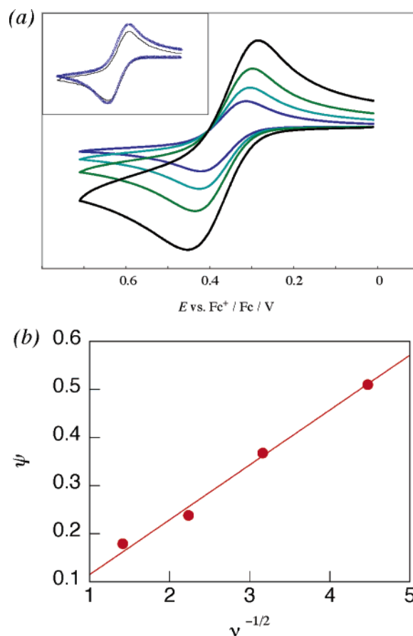
Figure 4. (a) Cyclic voltammograms of \text{HOAr-NH}_2 with \nu = 0.05, 0.1, 0.2 , and 0.5 \text{ V s}^{-1} . Inset: An overlay of the simulated (blue dots) and experimental CVs at 100 \text{ mV s}^{-1} . (b) Plot of \psi vs \nu^{-1/2} for \text{HOAr-NH}_2 (see eqs 3 and 4 in text).
