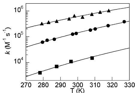
Figure 5. Temperature dependence of the rate constants for HOAr-py + [Fe(5,5′-Me 2 bpy) 3 ] 3+ (▲), HOAr-NH 2 + [N(tol) 3 ] •+ (●), and HOAr-im + [N(C 6 H 4 OMe) 3 ] •+ (■). The curve fits are to the non-adiabatic form of the Marcus equation (eq 15; see Discussion).
