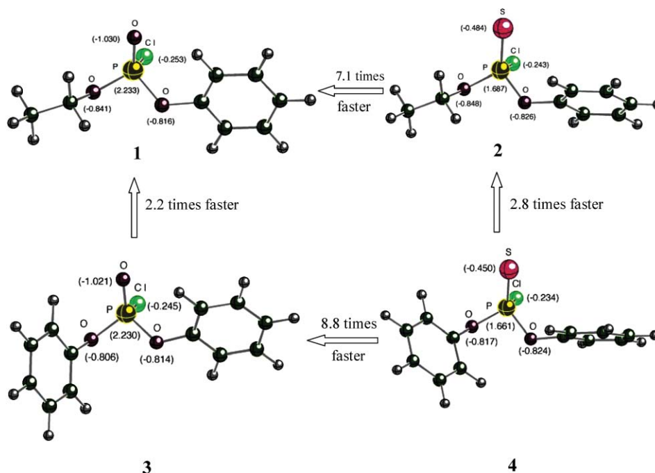
Fig. 1 The B3LYP/6-311+G(d,p) 10 geometries and NBO charges of 1 , 2 , 3 , 3a and 4 3c with Y = H. The relative rates are for unsubstituted aniline at 55.0 °C.
