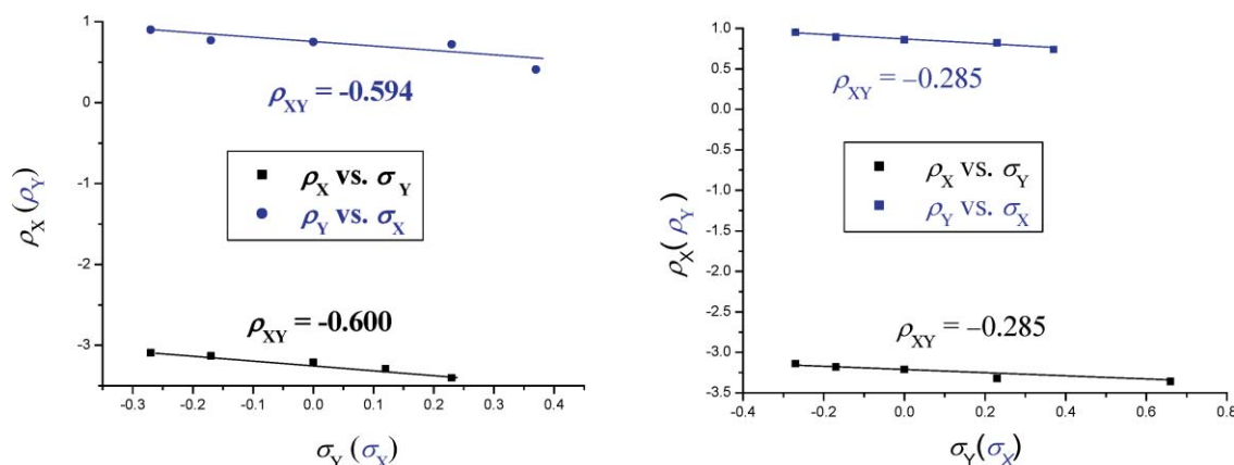
Fig. 4 The plots of \rho_{\text{X}} vs. \sigma_{\text{Y}} and \rho_{\text{Y}} vs. \sigma_{\text{X}} of the reactions of substrates, 1 and 2 , with X-anilines in acetonitrile at 55.0 °C.
