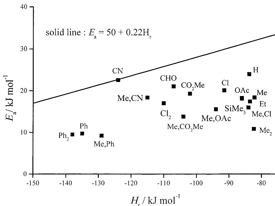
Fig. 8. Activation energies E_a for the addition of the 3,3,3-trifluoroacetyl radical to alkenes as a function of the reaction enthalpy H_{rx} . Solid line as expected for complete enthalpy control.
