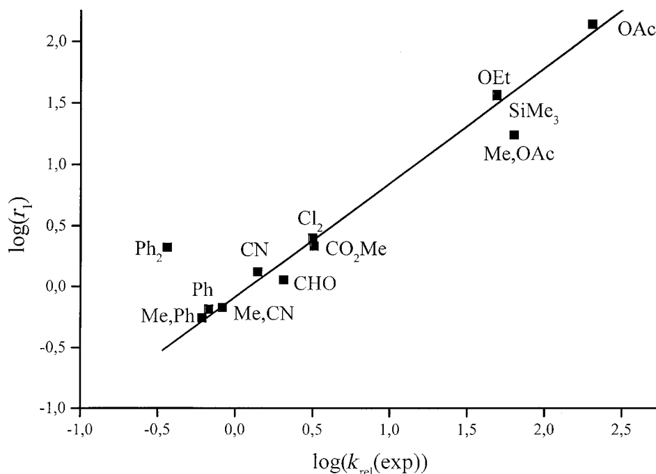
Fig. 11. Experimental co-polymerization parameters of methyl methacrylate vs. relative rate constants of the 2-(methoxycarbonyl)propan-2-yl radical
