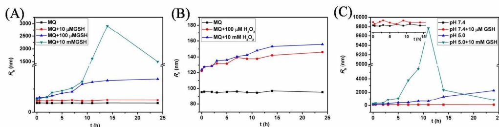
Figure 3. Changes in average diameters of blank PRDSP NPs as a function of time (A) in MQ with different concentrations of GSH; (B) in MQ with different concentrations of H 2 O 2 ; (C) in PBS at pH 7.4, pH 5.0 and conditions mimicking plasma and cancer cell environment monitored by DLS.
