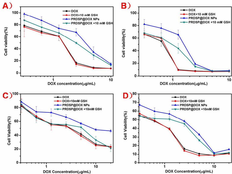
Figure 9. In vitro cytotoxicity of PRDSP@DOX NPs and free DOX·HCl at various DOX concentrations towards 10 mM GSH-pretreated or non-pretreated cells with different incubation time. (A) HeLa, 24 h; (B) HeLa, 48 h; (C) A549, 24 h; (D) A549, 48 h.
