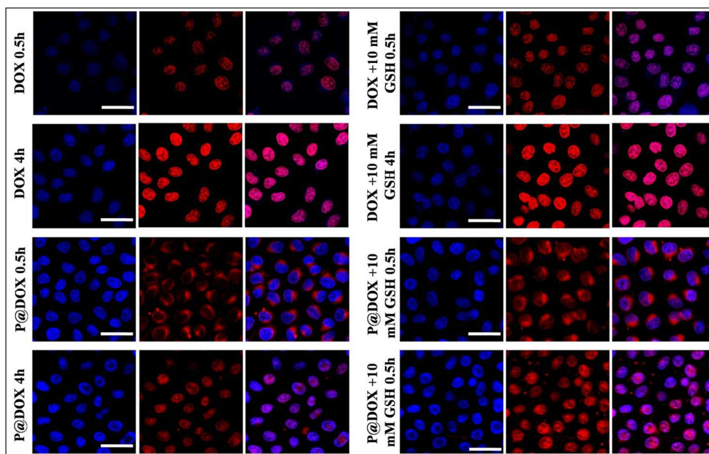
Figure 10. Cellular uptake of DOX and PRDSP@DOX NPs in the presence or absence of 10 mM GSH towards HeLa cells ( blue:Hoechst, red:DOX. Bar:50 \mu m).
