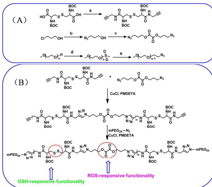
Scheme 2. Synthetic pathway for clickable monomers (A), ABA-type triblock copolymer PRDSP (B). Reagents and conditions: (a) propargyl amine, BOP, TEA, CH 2 Cl 2 , 0°C for 2 h, room temperature (rt) for 24 h; (b) NaN 3 , NaOH, H 2 O, 80°C for 48 h; (c) oxalylchloride, TEA, DMAP, CH 2 Cl 2 , 0°C to rt for 24 h; (d) mesyl chloride, TEA, DMAP, CH 2 Cl 2 , 0°C to rt for 24 h; (e) NaN 3 , DMF, 80°C for 24 h.
