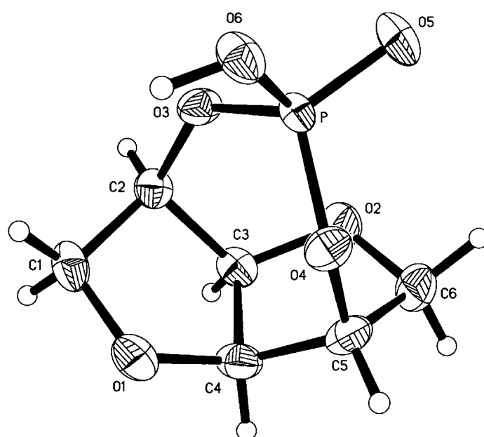
Figure 1 Molecular Structure of Compound ( 4 )
