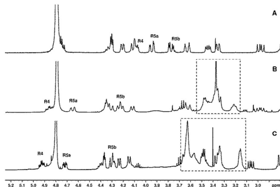
Fig. 3. ^1\text{H-NMR} (5.25 - 3.8 ppm, \text{D}_2\text{O} , 298 K) of A) vitamin B12, B) species 2 and C) species 3 . Signals enclosed in segmented boxes are those of 1,4,8,11-tetraazacyclotetradecane ( tacd ) and hexacyclen ( hacd ) respectively. Peaks labeled R4, R5a and R5b refer to resonances of the ribose sugar.
