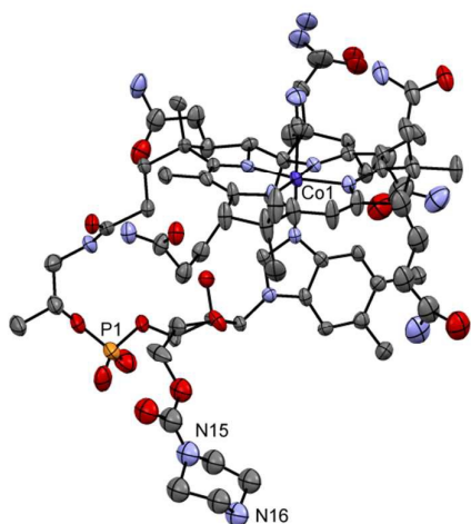
Fig. 1. X-ray structure of compound 1 with thermal ellipsoids drawn at 30% probability. Hydrogen atoms are omitted for clarity. Crystallographic details are summarized in ESI.
