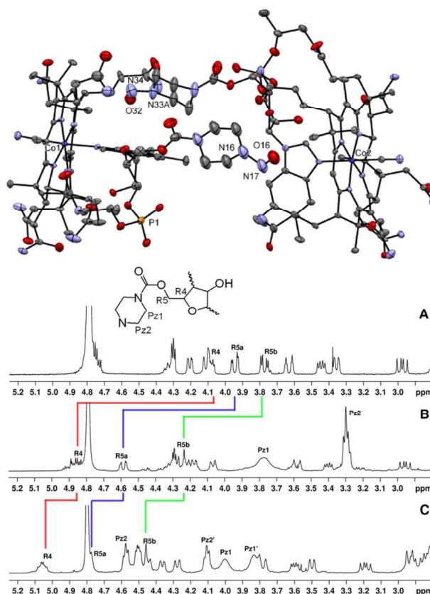
Fig. 1. X-ray structure of compound 1 with thermal ellipsoids drawn at 30% probability. Hydrogen atoms are omitted for clarity. Crystallographic details are summarized in ESI.
