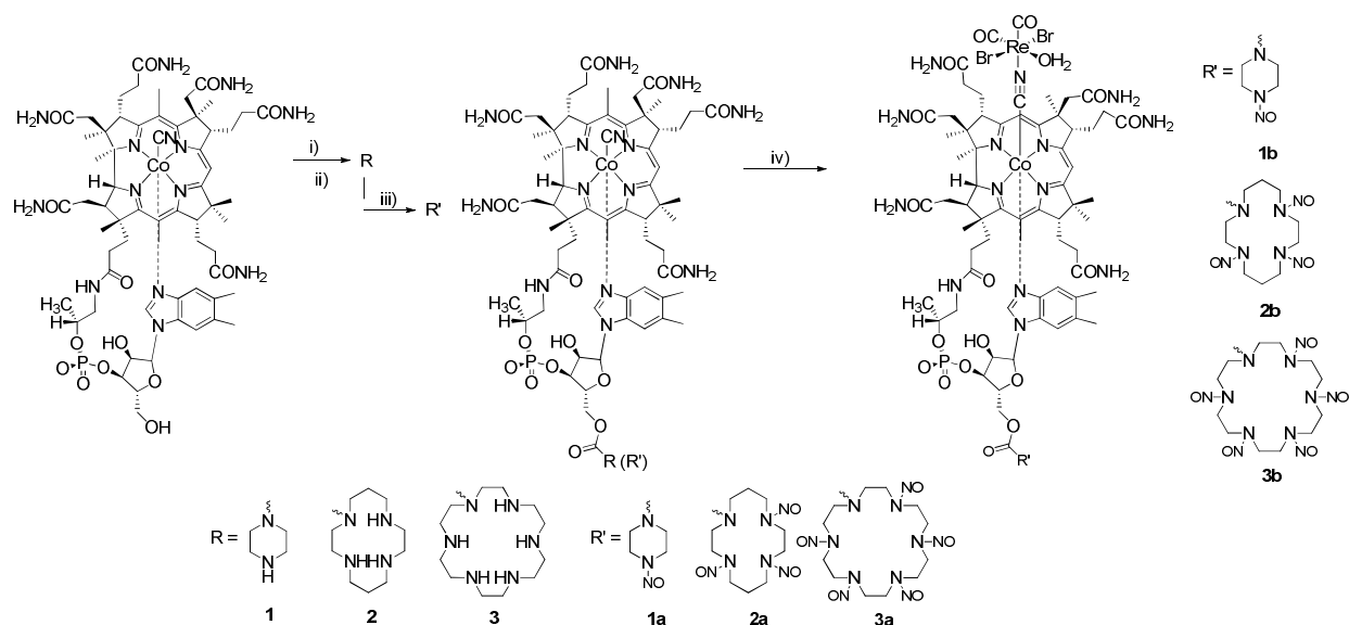
Scheme 1. Synthetic procedure to mixed CO/NO-releasing molecules. Conditions are: i) DMSO, CDT, 12h, 60 °C followed by ii) selected macrocycle; iii) AcOH, NaNO 2 , 2h, RT; iv) MeOH, [Et 4 N] 2 [Re(CO) 2 Br 4 ], N 2 , 1h, RT.
