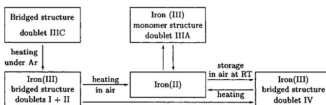
Scheme 1. Reaction scheme of iron(III) complexes with the 3,4-bis(decyloxy)benzyl-substituted 1,4,7-triazacyclononane ligand L deduced from Mössbauer spectroscopy.
