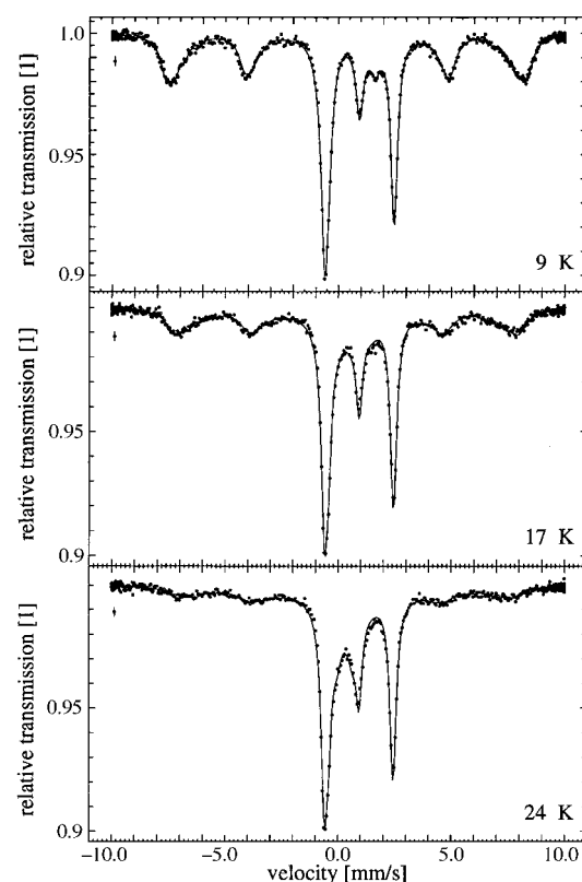
Figure 6. Mössbauer relaxation spectra at different temperatures observed for sample A \text{L} \cdot \text{FeCl}_3 \cdot 6\text{H}_2\text{O} before heating to 130 °C, and for all samples after the thermal transformation in air.
