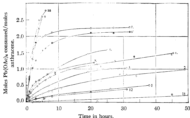
Fig. 1.—Effect of solvent on the oxidation of anthracene: 1, 99.9% HOAc (av. of 2); 2, 99% HOAc (av. of 5); 3, 98.9% HOAc; 4, 98.6% HOAc; 5, 95% HOAc-H 2 O; 6, 90% HOAc-10% H 2 O; 7, 85% HOAc-15% H 2 O; 8, 99% HOAc-0.5 M KOAc; 9, 50% HOAc-50% CH 3 OH; 10, 25% HOAc-75% CH 3 OH; 11, 50% HOAc-50% C 6 H 6 ; 12, 25% HOAc-75% C 6 H 6 .
