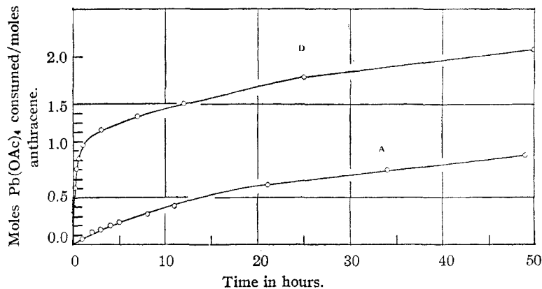
Fig. 2.—Oxidation of 9,10-dimethylantracene in 99% acetic acid.
