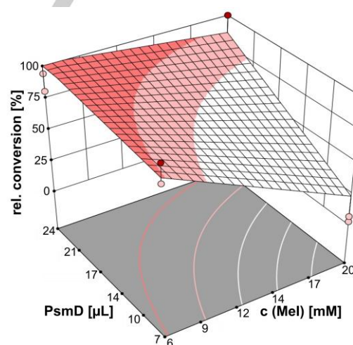
Figure 3. The diagram shows a 3D-cut of the hypersurface for the 4D-optimization. The red maximum corresponds to 100% conversion. For detailed information on the tested conditions for recycling optimization, see supporting information. The hypersurface is described by the equation: \text{conversion} = 125.5\% - 7.5898\% \mu\text{M}^{-1} \cdot c(\text{MeI}) + 0.5684\% \mu\text{L}^{-1} \cdot V(\text{PsmD}) - 0.0184\% \mu\text{L}^{-1} \cdot V(\text{CtHMT}) + 0.2074\% \mu\text{M}^{-1} \mu\text{g}^{-1} c(\text{MeI}) \cdot V(\text{PsmD}) + 0.0058\% \mu\text{M}^{-1} \mu\text{L}^{-1} \cdot c(\text{MeI}) \cdot V(\text{CtHMT}) - 0.00418\% \mu\text{L}^{-1} \mu\text{L}^{-1} \cdot V(\text{PsmD}) \cdot V(\text{CtHMT}) .
