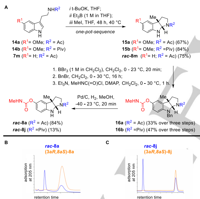
Scheme 3. A Synthesis of the racemic standard compounds 8a,j+m . B+C HPLC-traces for the ee-analytics of compounds 8a+j (in blue - racemic standard, in orange - compounds obtained after enzymatic methylation with >99% ee; for details see supporting information).
