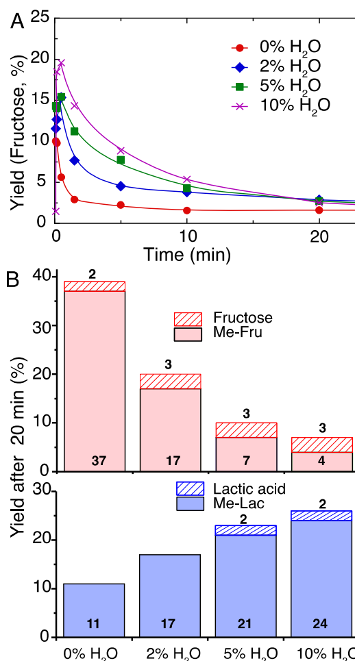
Fig. 8 (A) Fructose formation from glucose in the presence of different amounts of water. (B) Methyl fructoside and methyl lactate formation from glucose within 20 minutes of reaction time in the presence of varying amounts of water. Conditions: 120 mg glucose, 50 mg HT Sn-Beta (150) catalyst, MW reactor for the indicated time at 160 °C in the presence of indicated amounts of water (% v/v).
