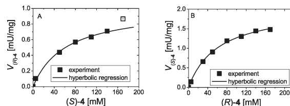
Fig. 3 Formation rates of ( R )- 4 from enantiopure ( S )- 4 (A) and formation rates of ( S )- 4 from enantiopure ( R )- 4 (B). Reaction conditions: ( R )- or ( S )- 4 (0–170 mM), 25 mM acetaldehyde, 50 mM TEA buffer, 0.5 mM ThDP, 2 mM \text{Mg}^{2+} , wtBFD (51 \text{U}_{2\text{-HPP}} \text{mL}^{-1} , 6 \text{mg mL}^{-1} wtBFD) at pH 7.5 and 25 °C. Data points are average values of duplicates.
