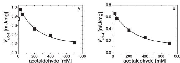
Fig. 4 Formation rates of ( R )- 4 from 30 mM of enantiopure ( S )- 4 (A) and formation rates of ( S )- 4 from 30 mM of enantiopure ( R )- 4 (B) as a function of the acetaldehyde concentration (0–700 mM). Reactions were carried out in 50 mM TEA buffer, 0.5 mM ThDP, 2 mM \text{Mg}^{2+} , wtBFD (21 \text{U}_{2\text{-HPP}} \text{mL}^{-1} (2.5 \text{mg mL}^{-1} wtBFD) for ( S )- 4 and 33 \text{U}_{2\text{-HPP}} \text{mL}^{-1} (4 \text{mg mL}^{-1} wtBFD) for ( R )- 4 ), at pH 7.5 and 25 °C. Data points are average values of duplicates.
