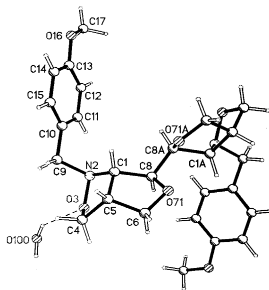
Fig. 2 Molecular plot of (1' S ,5' R ,8' S )-8,8'-bi[2'-( p -methoxybenzyl)-3',7'-dioxa-2'-azabicyclo[3.3.0]octane] 8b . Selected bond lengths (Å): C1–N2 1.456(5), C1–C8 1.513(5), C1–C5 1.553(5), N2–O3 1.446(3), N2–C9 1.468(5), C3–C4 1.446(5), C4–C5 1.519(6), C5–C6 1.505(6), C6–O71 1.340(6), C8–C8 a 1.484(7), C8–O71 1.515(7); selected bond angles (°): N2–C1–C8 112.5(3), N2–C1–C5 107.6(3), C8–C1–C5 103.7(3), O3–N2–C1 103.0(3), O3–N2–C9 109.5(2), C1–N2–C9 112.5(3), C4–O3–N2 107.5(3), O3–C4–C5 105.7(3), C6–C5–C4 115.0(4), C6–C5–C1 103.8(3), C4–C5–C1 102.3(3), O71–C6–C5 106.4(4), C8 a –C8–C1 115.1(4), C8 a –C8–O71 98.4(3), C1–C8–O71 99.5(4), C6–O71–C8 106.1(4). a Symmetry transformations used to generate equivalent atoms: – x , y , – z + 1.
