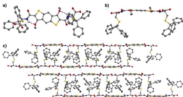
Fig. 2 a) Top view of the X-ray structure of 6 showing the presence of the quasi-pentacyclic core through the hydrogen bonding (dashed line) between NH and OMe. b) side view and c) solid state packing structure of 6 viewed along the crystal a-axis. All H atoms, except NH, have been removed for clarity. (C – grey, H – white, O – red, N – blue, S – yellow) – CCDC: 2006236.
