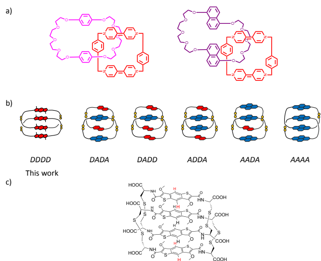
Scheme 1 a) The previously published all-donor [2]catenanes by Stoddard group; b) the arrangement described in this paper along with the other types of [2]catenanes stacking published by Sanders group (red - \pi -donor, dialkoxyanaphthalene, blue - \pi -acceptor, naphthalenediimide) and c) the chemical structure of the all-donor aromatic [2]catenane synthesised in the paper.
