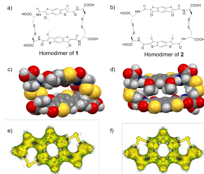
Fig. 7 Chemical structures (a,b) and overlapping spheres optimized geometries of homodimers of 1 and 2 (c, d). Anisotropy induced current densities (ACID) plots (isovalue 0.05 e/bohr 2 ) of the BDT and iBDT cores (e,f).
