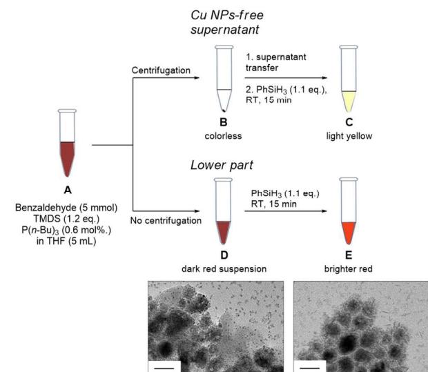
Scheme 2 – Leaching test and TEM of the supernatants (D) and (E), black bar is 50 nm
