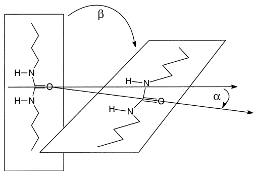
Figure 8. Colinearity angle \alpha and dihedral \text{N}-\text{C}-\text{O}\cdots\text{H} angle \beta of two hydrogen-bonded urea fragments.
