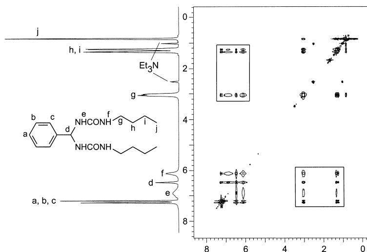
Figure 11. NOESY spectrum of 1 at a concentration of 27.2 mM in CDCl 3 .
