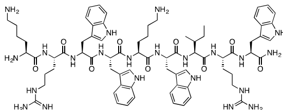
Figure 1. HHC10 Cationic Amphiphilic Peptide developed by Hancock et al. 5
