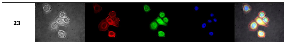
Figure 5. Fluorescence micrographs of MCF7 cells with 20 \mu M of BODIPY-CAPs 19, 20, 21, 22 and 23. Blue fluorescence of DAPI (4',6-DiAmidinoPhenylIndole) stained nuclei and red fluorescent components of the cytoskeleton were obtained by marking with Rhodamine Phalloidin. Green (BODIPY) fluorescent Cationic Amphiphilic Peptides showed their cellular uptake and localisation. Pictures were merged to visualise the localisation of the fluorescent peptides inside the cell thus confirming their cell penetrating properties. The white scale bar in the right figure of each frame is 10 \mu m.
