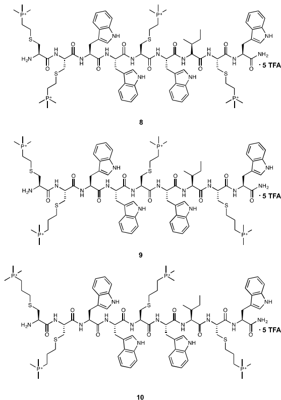
Figure 2. HHC10 derivatives with the phosphonium charged amino acids
