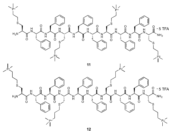
Figure 3. Phosphonium Analogues of the bactericidal peptide KFFKFFKFFK
