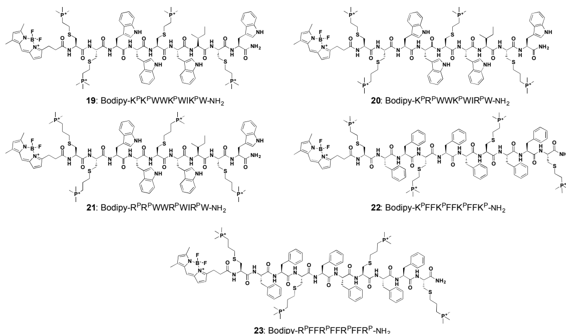
Figure 4. Green fluorescent phosphonium peptides.
