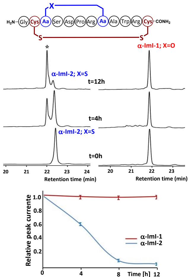
Figure 3. Oxidative stability studies on \alpha -Iml-1 and \alpha -Iml-2 under 0.1% hydrogen peroxide. After 12 hours, almost all \alpha -Iml-2 is oxidized, whereas no oxidation by-products of \alpha -Iml-1 were observed. * refers to \alpha -Iml-2 in which thioether is oxidized to sulfoxide.
