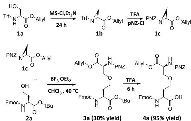
Scheme 2 Chemical synthesis of ether-containing diaminodiacids 4a
