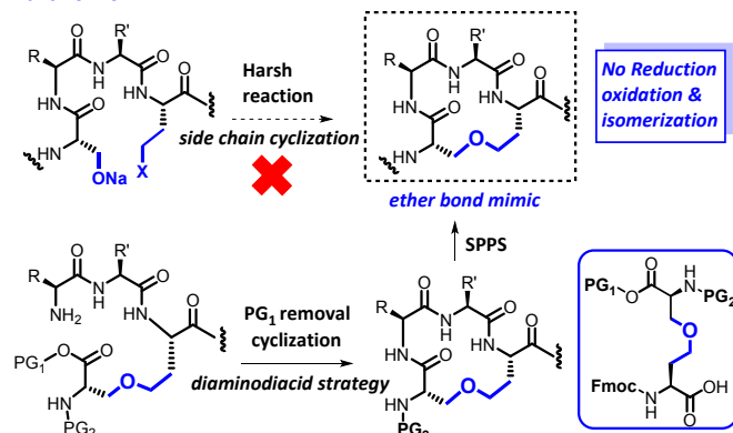
Scheme 1 Diaminodiacid strategy enabled the development of the first example of cysteine-rich peptide exploiting the ether-bond as disulfide-bond mimic. These ether-containing peptide mimics exhibit significant stability to both reduction and oxidation conditions.
