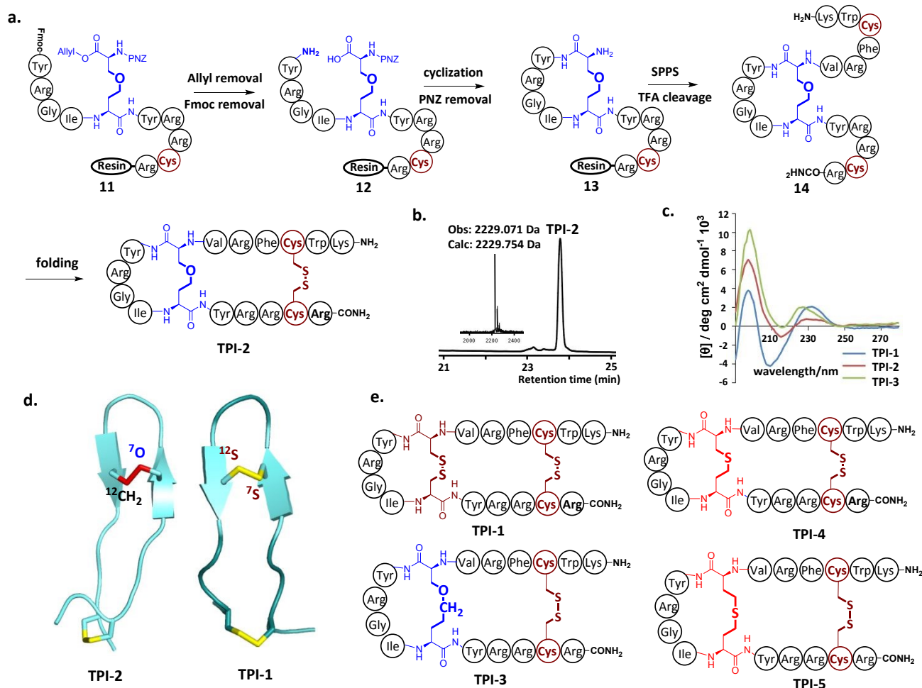
Figure 2. a. Solid-phase synthetic route for the preparation of ether-containing TPI-2 using diaminodiacid 4a . b. HPLC traces and ESI-MS analysis of purified refolded TPI-2 . c. CD spectra of TPI-1 , TPI-2 and TPI-3 in water. d. NMR structure of TPI-1 (right) and ether-containing analogue TPI-2 (left). Disulfides are shown in yellow and the ether bond in red. e. The structure of side-chain extended ether-containing TPI-3 and different lengths of thioether linkage substituted TPI-1 derivatives TPI-4 and TPI-5 .
