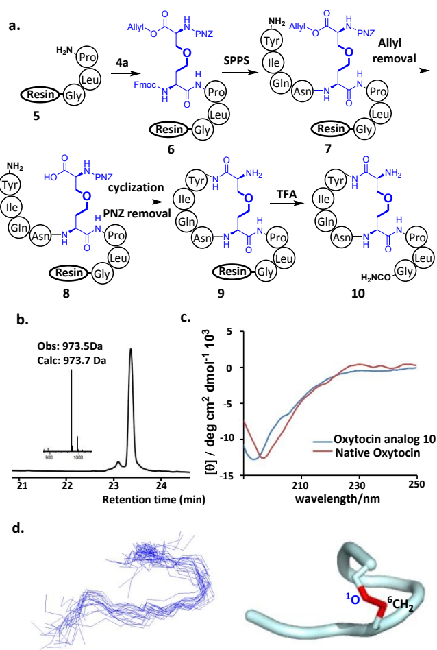
Figure 1. a. Synthetic route for the preparation of oxytocin analog using diaminodiacid 4a . b. HPLC traces and ESI-MS analysis of purified oxytocin analog. c. CD spectra of oxytocin analogue in water. d. Backbone ensembles of 20 lowest-energy NMR structures of oxytocin analog 10 (left) and a ribbon representation of 10 (right). The C-O bridge is shown in red.
