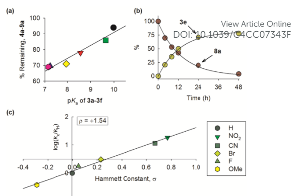
Figure 1. (a) A comparison of GSH-mediated decomposition of 4a-9a monitored by HPLC analysis of reaction mixtures after 4 h and the reported pK_a s of the corresponding leaving groups, 3a-3f ; (b) Time courses of GSH-mediated decomposition of 8a and formation of 3e were monitored by HPLC analysis. Curve fitting gave rate constants for decomposition of 8a and formation of 3e ; (c) Linear Free Energy Relationship Analysis of \log(k_x/k_f) obtained from rate constants for thiol-mediated decomposition of 8a-8f (Table 3) and Hammett constants.
