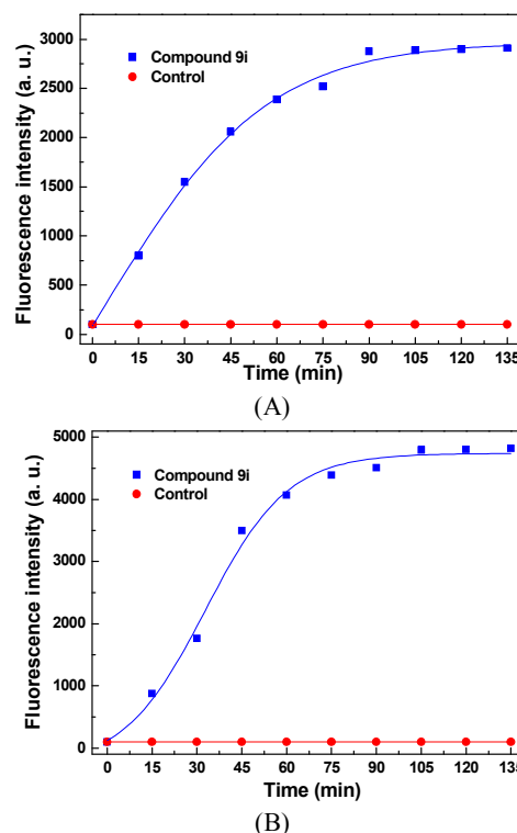
Fig. 2 Bacterial membrane permeabilization of compound 9i (12 \times MIC) against: (A) MRSA; (B) B. proteus .
