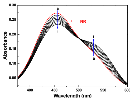
Fig. 6 UV absorption spectra of NR in the presence of DNA at pH 7.4 and room temperature. c(\text{NR}) = 2 \times 10^{-5} mol/L, and c(\text{DNA}) = 0-3.81 \times 10^{-5} mol/L for curves a-i respectively at increment 0.48 \times 10^{-5} .
