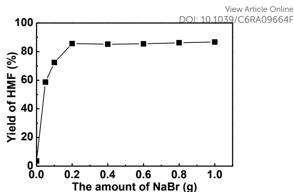
Fig. 5. Influence of NaBr amounts. Reaction conditions: 0.1 g fructose, 50 mg Nb-NTMPA, 2 g DMA, reaction time 1.5 h, reaction temperature 100 °C.
