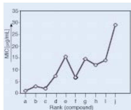
Figure 13. Correlation of relative abundance of vancomycin dimers (a–j, Figure 12 and Table 5), with antibacterial activity (MIC, average of the vancomycin susceptible strains listed in Table 5).
