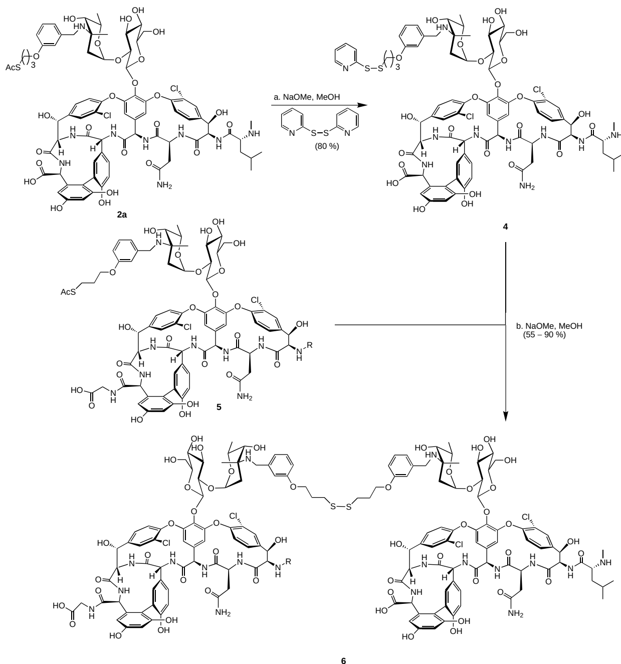
Scheme 2. Formation of the vancomycin-derived heterodimers 6 . a) NaOMe (10.0 equiv), pyS-Spy (5.0 equiv), MeOH, 23 °C, 30 min, 80 %; b) 4 (1.0 equiv), 5 (1.1 equiv), NaOMe (10.0 equiv), MeOH, 23 °C, 45 min, 55 – 90 %. See Table 4 for definitions of R. Compounds are designated and referred to as 6 -(xxx) where xxx is the three letter code for the amino acid represented by R. py = pyridine.
