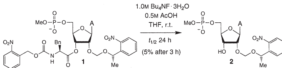
Scheme 2. Model Investigation to Determine the Stability of Protected Aminoacylated Nucleotide Derivatives under the Conditions Required for the Removal of Fluoride-Labile Protecting Groups
