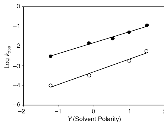
Fig. 1 Grunwald–Winstein plot of \log k vs. Y^{11} 3 (●) r = 0.996 and 7 (○) r = 0.993 .
