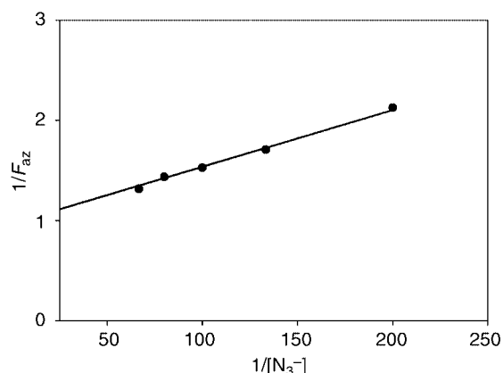
Fig. 3 Azide trap ( 1/F_{\text{az}} vs. 1/[\text{N}_3^-] ) for 7 . Solvent 50 : 50 acetonitrile–MeOH. Ionic strength was maintained at 0.015 M with \text{NaClO}_4 ( r = 0.995 ). Product ratios were calculated from ^1\text{H} proton NMR analysis.
