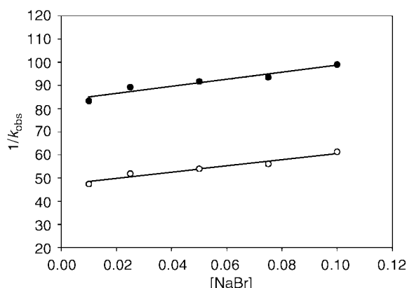
Fig. 2 Common ion effect 1/k_{\text{obs}} vs. [\text{NaBr}] in 80% acetonitrile and 20% water for 1 (●) r = 0.964 and 7 (○) r = 0.977 . 1/k_{\text{obs}} for 7 divided by 50 for ease of presentation.
