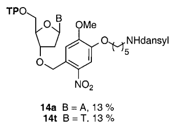
Scheme 2. Preparation of 14a and 14t.
