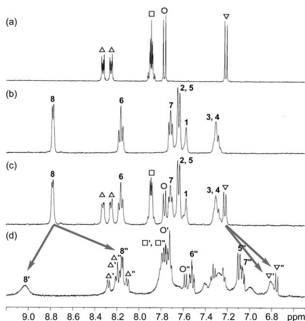
Fig. 3 ^1\text{H} NMR spectra in \text{CD}_3\text{OD}-\text{D}_2\text{O} (9 : 1 v/v) (400 MHz) at 23 °C. [alizarin] = 2.4 mM, [ 1\cdot\text{Zn} ] = 2.4 mM; (a) alizarin, (b) 1\cdot\text{Zn} , (c) alizarin plus 1\cdot\text{Zn} , (d) alizarin plus 1\cdot\text{Zn} with PPI. The spectrum of (d) was obtained after (solid \text{PPI} )-liquid (2.4 mM of alizarin and 1\cdot\text{Zn} in \text{CD}_3\text{OD}-\text{D}_2\text{O} (9 : 1 v/v)) two-phase extraction in view of the low solubility of \text{PPI} under NMR detectable conditions.
