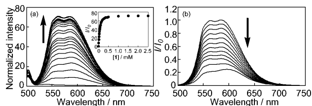
Fig. 1 (a) Change in the fluorescence spectra of ARS (50 μM) upon adding 1 in MeOH–10 mM HEPES (1 : 1 v/v) containing 10 mM NaCl at pH 7.4 at 25 °C, \lambda_{\text{ex}} = 501 nm; (b) Change in the fluorescence spectra of ARS (50 μM) in the presence of 1 (250 μM) upon adding Zn II in MeOH–10 mM HEPES (1 : 1 v/v) containing 10 mM NaCl at pH 7.4 at 25 °C, \lambda_{\text{ex}} = 480 nm. I 0 is fluorescence intensity under the Zn II -free conditions.
