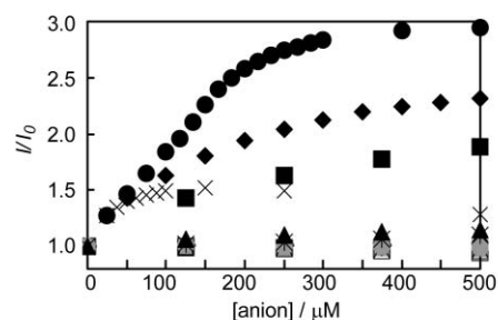
Fig. 4 Plots of fluorescence intensity at 586 nm of \text{ARS} (50 \mu\text{M} ) and 5 equiv. of 1\cdot\text{Zn} as a function of anion concentration. The measurements were carried out in \text{MeOH}-10 mM \text{HEPES} (1:1 v/v) containing 10 mM \text{NaCl} at pH 7.4 at 25 °C, \lambda_{\text{ex}} = 480 nm.
