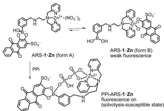
Scheme 2 A plausible mechanism for the \text{PPI} -induced fluorescence enhancement.
