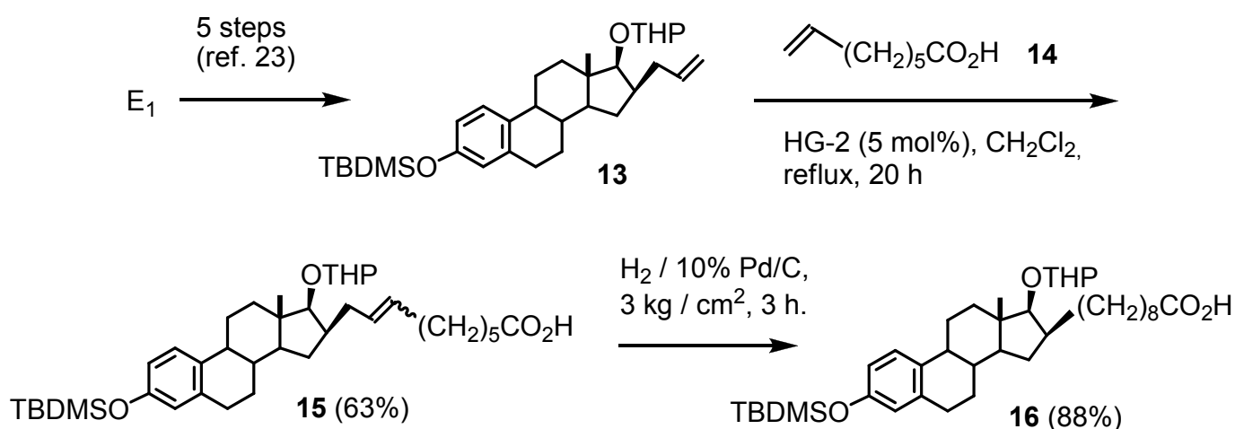
Scheme 2. Synthesis of left half 16
