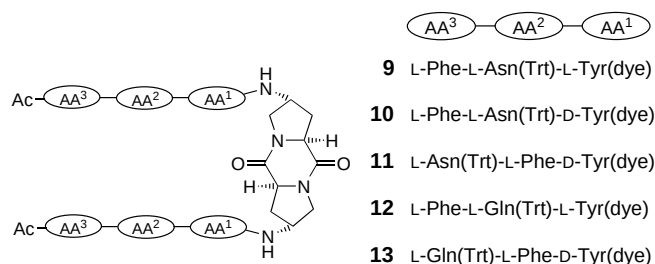
Figure 2. Diketopiperazine receptor prototypes 9 – 13 .
