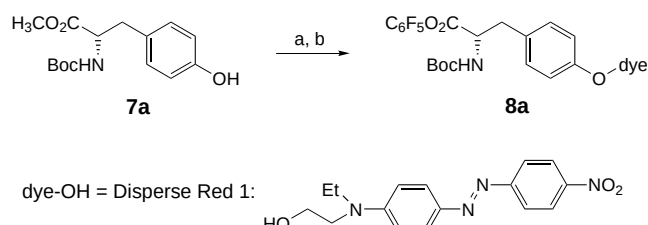
Scheme 2. Synthesis of N -Boc-L-Tyr(dye)- \text{OC}_6\text{F}_5 8a : a) Disperse Red 1, \text{PPh}_3 , \text{DEAD} , toluene, 72%; b) i) \text{NaOH} , \text{MeOH} , \text{THF} , \text{H}_2\text{O} ; ii) \text{C}_6\text{F}_5\text{OH} , \text{EDC} , \text{CH}_2\text{Cl}_2 , 95%.
