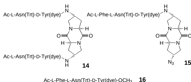
Figure 3. Receptor fragments 14 – 16 .
