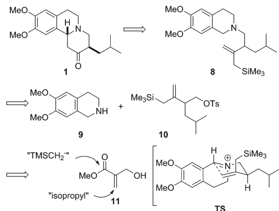
Scheme 2. Retrosynthetic Analysis
