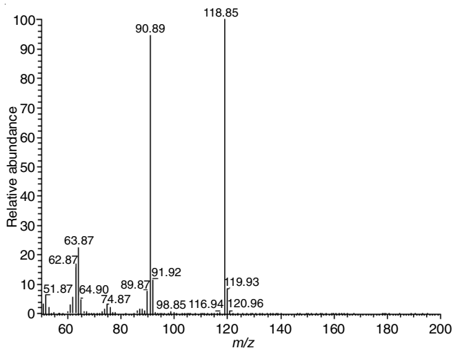
Fig. 4. MS spectrum of component at RT = 5.95 min
