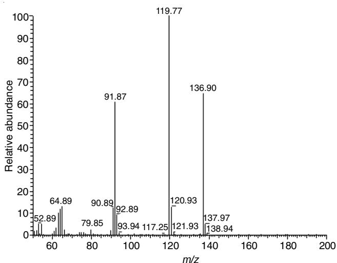
Fig. 5. MS spectrum of component at RT = 8.34 min
