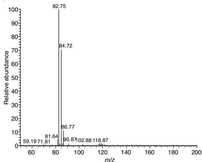
Fig. 2. MS spectrum of component at RT = 2.17 min
