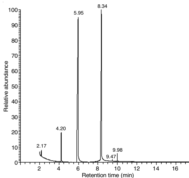
Fig. 1. GC spectrum of catalytic dehydration product of \text{ZrO}_2 supported phosphoric acid
