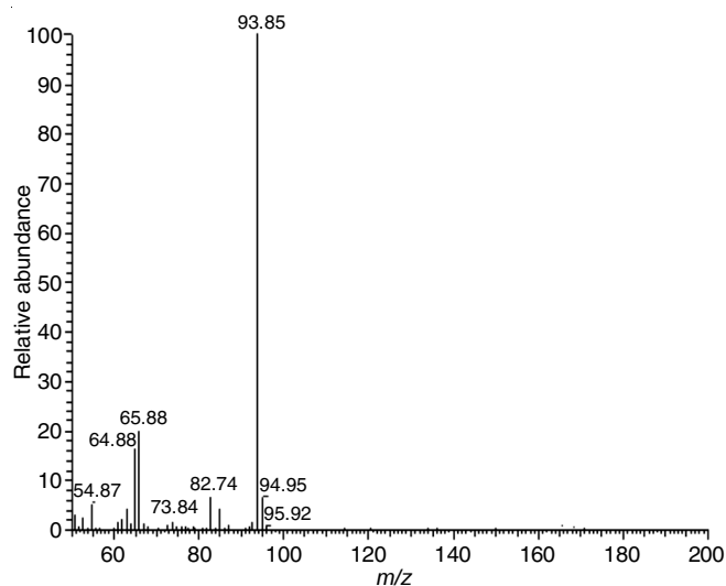
Fig. 3. MS spectrum of component at RT = 4.20 min
