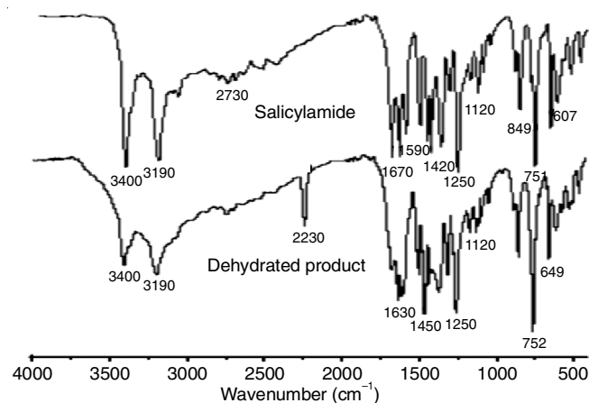
Fig. 8. FT-IR spectra of salicylamide and its catalytic dehydration product
