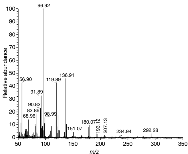
Fig. 6. MS spectrum of component at RT = 9.47 min
