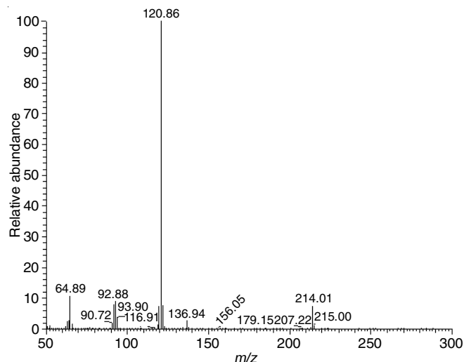
Fig. 7. MS spectrum of component at RT = 9.98 min
