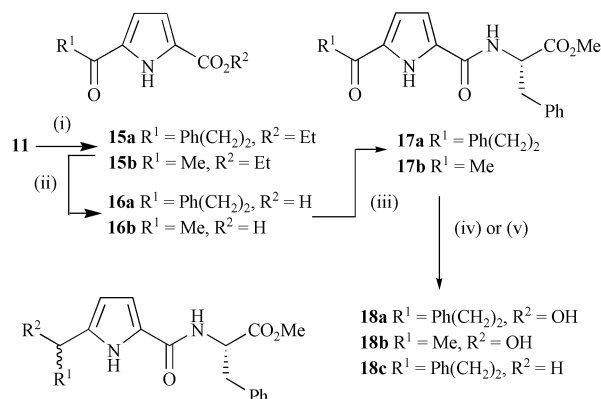
Scheme 4 Reagents and conditions: (i) ZnCl 2 , 1,2-DCE, 50 °C, 1 h and Ph(CH 2 ) 2 COCl ( 15a , 35%) or AcCl ( 15b , 37%); (ii) KOH, 2 : 1 H 2 O–THF, 40–50 °C, 2 h ( 16a , 86%), ( 16b , 93%); (iii) L-PheOMe·HCl, EDCI, HOBT, DIEA, CH 2 Cl 2 , rt, 16 h ( 17a , 70%), ( 17b , 91%); (iv) Zn(BH 4 ) 2 , ether, 0 °C, 1 h ( 18a , 21%), ( 18c ); (v) LiBH 4 , ether, −78 °C, 1 h, then rt, 1 h ( 18b , 46%).
