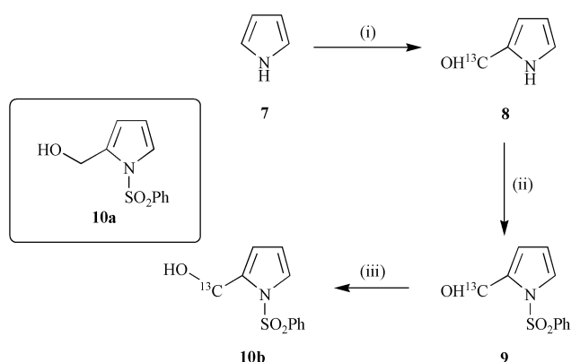
Scheme 2 Reagents and conditions: (i) POCl 3 , 13 C-DMF, 1,2-DCE, reflux, 15 min, then CH 3 CO 2 Na·3H 2 O (aq) , reflux, 15 min (59%); (ii) PhSO 2 Cl, 30% NaOH (aq) , Bu 4 NI, CH 2 Cl 2 , rt, 30 h (91%); (iii) Zn(BH 4 ) 2 , Et 2 O, 0 °C, 30 min (90%).
