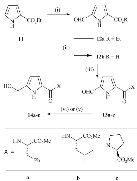
Scheme 3 Reagents and conditions: (i) POCl 3 , DMF, 1,2-DCE, reflux, 15 min, then CH 3 CO 2 Na·3H 2 O, reflux, 15 min (61%); (ii) KOH, H 2 O, 40–50 °C, 2 h (60%); (iii) EDCI, HOBT, DIEA, CH 2 Cl 2 , rt, 16 h and either L-PheOMe·HCl ( 13a , 71%), L-LeuOMe·HCl ( 13b , 61%), or L-ProOMe·HCl ( 13c , 74%); (vi) Zn(BH 4 ) 2 , ether, 0 °C, 1 h ( 14a , 57%), ( 14b , 42%), ( 14c , 24%); (v) LiBH 4 , ether, −78 °C, 1 h ( 14b , 66%).
