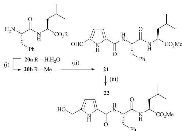
Scheme 6 Reagents and conditions: (i) CH 2 N 2 , THF, rt, 15 h; (ii) 12b , BOP, DIEA, CH 2 Cl 2 , rt, 16 h (52% yield over two steps); (iii) LiBH 4 , THF, –78 °C, 1 h, then rt, 1 h (66%).
