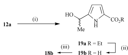
Scheme 5 Reagents and conditions: (i) MeLi, THF, –23 °C, 5 h (95%); (ii) NaOH, 1 : 1 THF–H 2 O, 40–50 °C, 24 h (17%); (iii) L-PheOMe·HCl, EDCI, HOBT, DIEA, CH 2 Cl 2 , rt, 16 h (54%).
