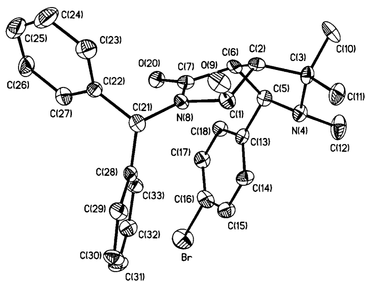
Fig. 6. X-Ray crystal structure of hydroxy lactam (±)- 25 . Arbitrary numbering. Atomic displacement parameters obtained at 293 K are drawn at the 50% probability level.
