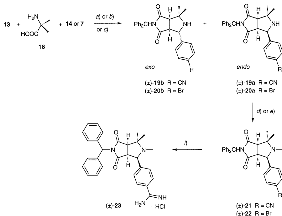
Scheme 3. Synthesis of Inhibitor ( \pm )- 23
