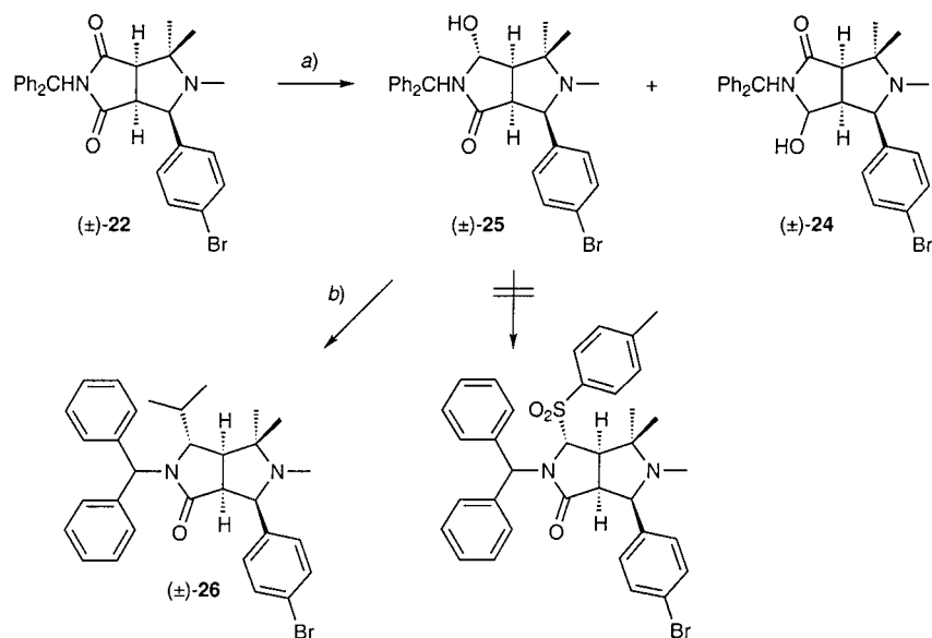
Scheme 4. Introduction of the i -Pr Side Chain into (±)- 22
