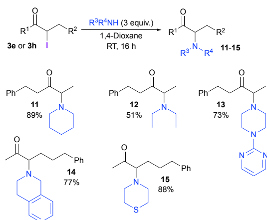
Scheme 4 Regioselective synthesis of \alpha -amino ketones.
