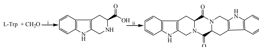
Scheme 2 Synthetic route of the preparation of THPDTP1. i) Sulfuric acid (1 M); ii) EDC, N-hydroxybenzotriazol, DMF, N-methylmorpholine.
