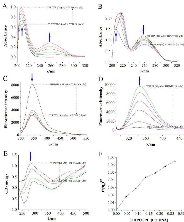
Fig. 8 Intercalation of THPDTPi towards CT DNA in vitro . (A) UV spectrum of 0.9 \mu\text{M} of THPDTPi with increased amount of CT DNA; (B) UV spectra of 200 \mu\text{M} of CT DNA with increased amount of THPDTPi; (C) fluorescence spectra of 0.18 \mu\text{M} of THPDTPi with increased
