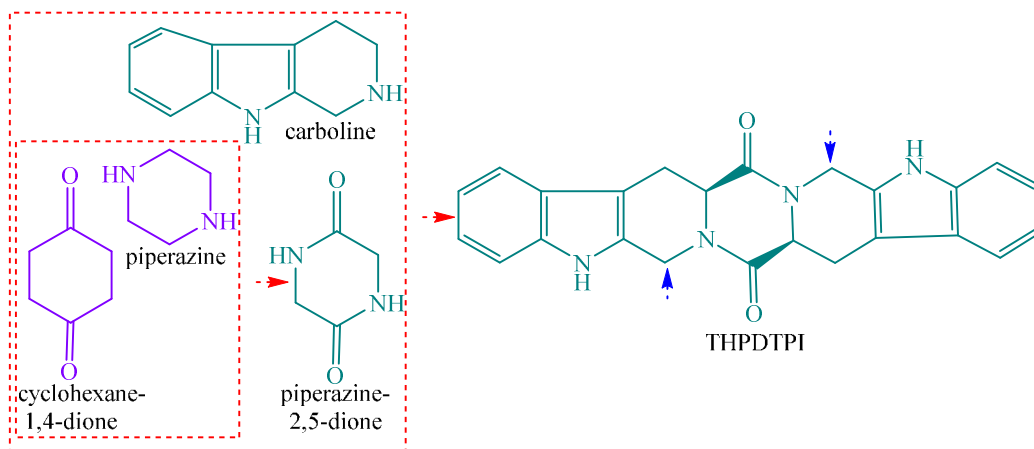
Scheme 1 Design of novel DNA intercalator, heterocycle THPDTP1, wherein the blue arrowheads represents the easy modifying positions.
