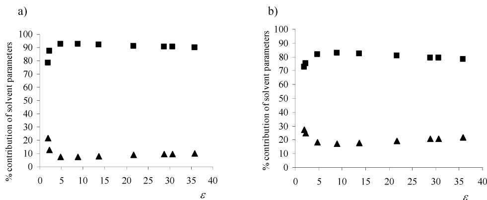
Fig. 8 Percent contribution of electrostatic (■) and cavitational energy interactions (▲) on the enolization (a) and ketonization (b) reaction of 2-NCH in solvents of different permittivity, \epsilon .
