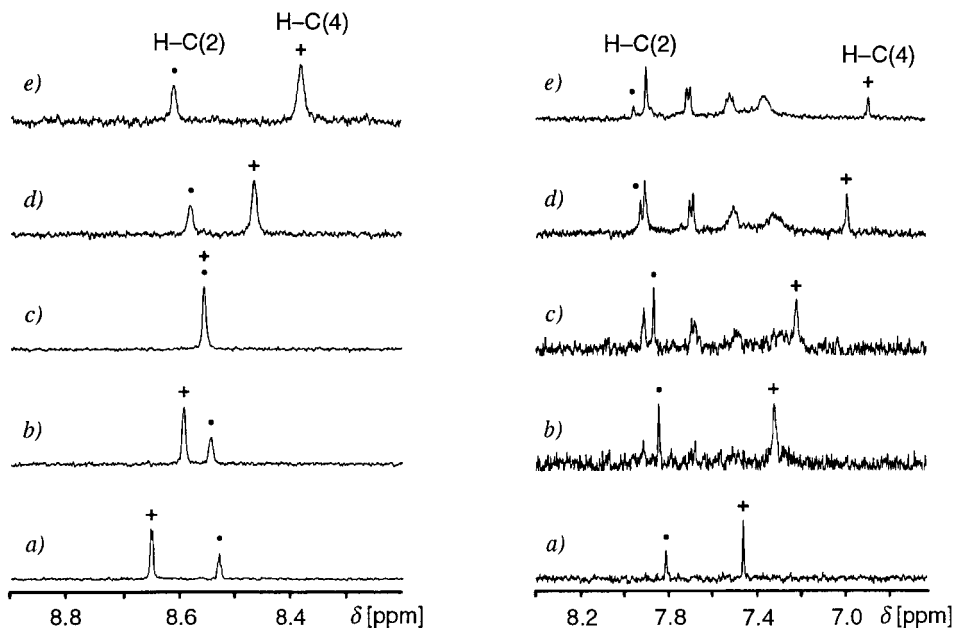
Fig. 5. Two examples of ^1\text{H} -NMR titrations with isophthalates in \text{D}_2\text{O} containing \text{Na}_2\text{B}_4\text{O}_7 (5 mM) at 300 K, pH 9.2. Left: Part of the ^1\text{H} -NMR spectrum of 25b (0.5 mM) alone (a) and in the presence of receptor at [\mathbf{3}] = 0.12 (b), 0.21 (c), 0.50 (d), and 1.0 (e) mM. Right: Part of the ^1\text{H} -NMR spectrum of 26b (0.2 mM) alone (a), and in the presence of receptor at [\mathbf{3}] = 0.049 (b), 0.084 (c), 0.20 (d), and 0.41 (e) mM.
