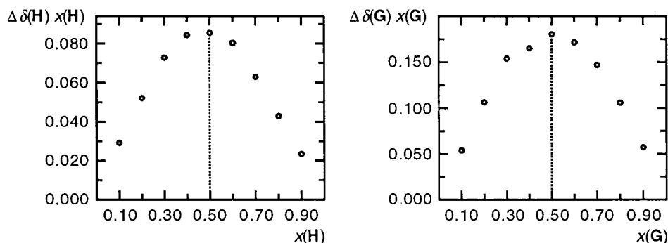
Fig. 7. Job plots for the complex formed between AMP ( 28 ) and 3 in \text{D}_2\text{O} containing Tris/HCl (5 mM) at 300 K, pH 8.3. The total concentration c_0(\text{H}) + c_0(\text{G}) was kept constant at 2 mM. The host signal H-C(2') (left graph) and the guest signal H-C(2) (right graph) were followed. For further definitions, see Caption to Fig. 3.
