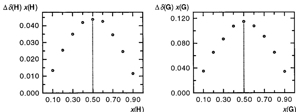
Fig. 4. Job plots for the complex formed between 3 and 25b in \text{D}_2\text{O} containing \text{Na}_2\text{B}_2\text{O}_7 (5 mM) at 300 K, pH 9.2. The total concentration c_0(\text{H}) + c_0(\text{G}) was kept constant at 2 mM. The host signal H–C(2') (left graph) and the guest signal H–C(4) (right graph) were followed. For further definitions, see Caption to Fig. 3.
