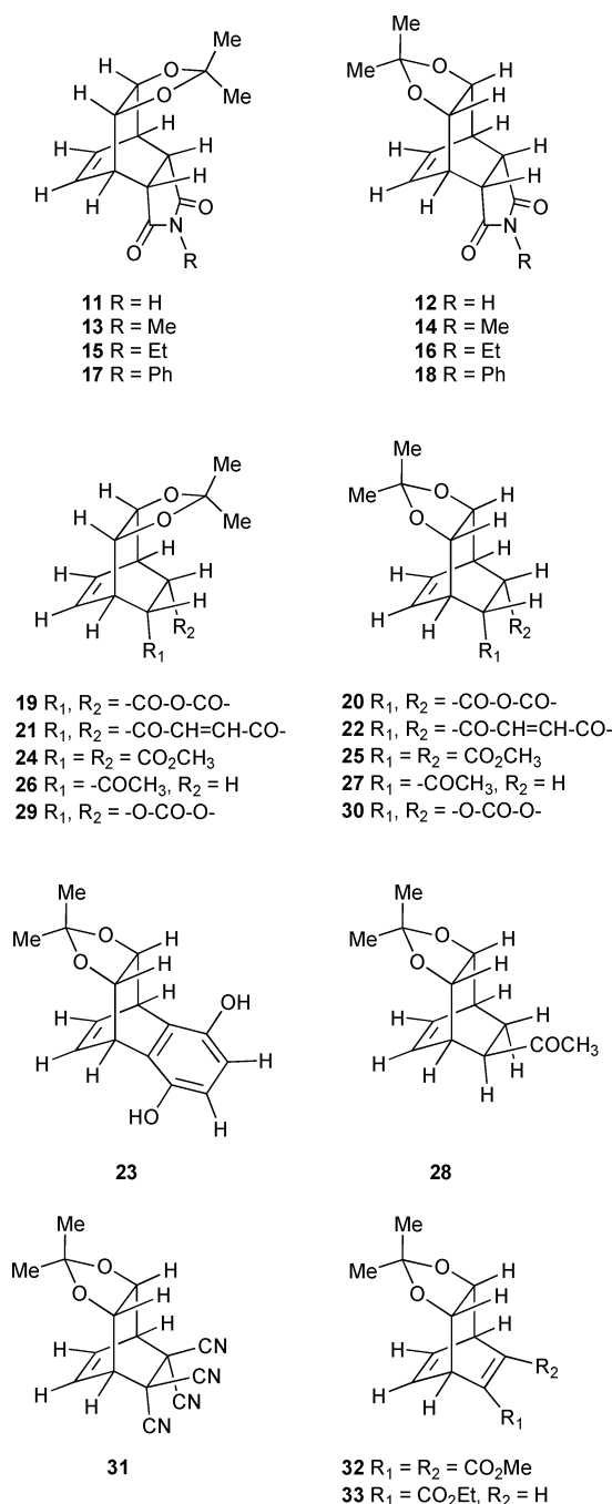
Fig. 2 Adducts derived from diene 6a and various ethylenic and acetylenic dienophiles.
