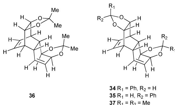
Fig. 3 Dimeric products from acetonides.
