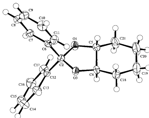
Fig. 6. ORTEP Plot [26] of the molecular structure of 37a (major conformation only shown; disorder not shown; arbitrary numbering of the atoms; 50% probability ellipsoids)
