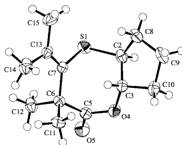
Fig. 4. ORTEP Plot [26] of the molecular structure of 23 (arbitrary numbering of the atoms; 50% probability ellipsoids)
