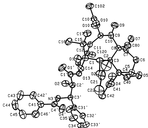
Fig. 1. ORTEP drawing of 2-debenzoyl, 2-acetoxy paclitaxel showing the atomic labeling scheme. The thermal ellipsoids were drawn at 50% probability level.
