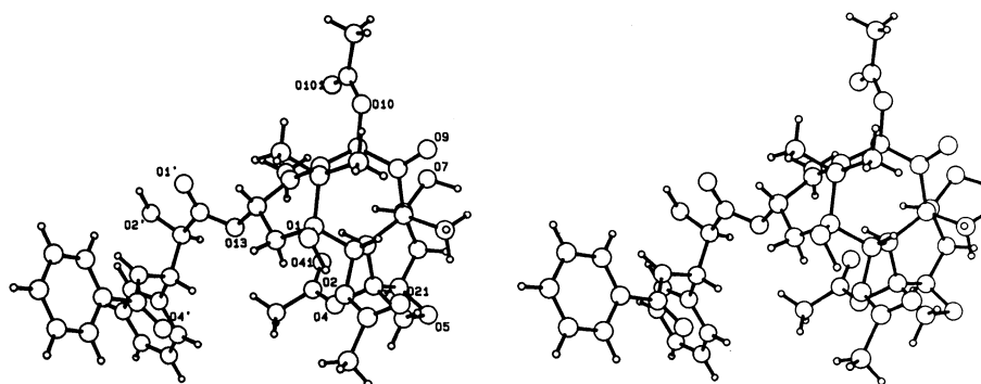
Fig. 2. Stereoscopic view of X-ray structure of 2-debenzoyl, 2-acetoxy paclitaxel.
