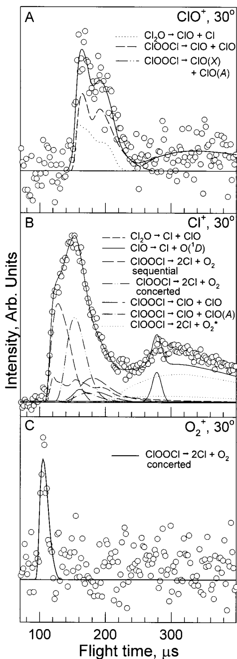
Figure 1. Time-of-flight (TOF) distributions for products from ClOOCl photolysis at 248 nm. TOF spectra were collected at a detector angle of 30° for (A) ClO + , (B) Cl + , and (C) O 2 + fragments. The contribution in B from the ClO + ClO product channel arises from fragmentation to Cl + in the ionizer, and the contribution from the ClO + ClO(A) channel arises from predissociation of the ClO(A).
