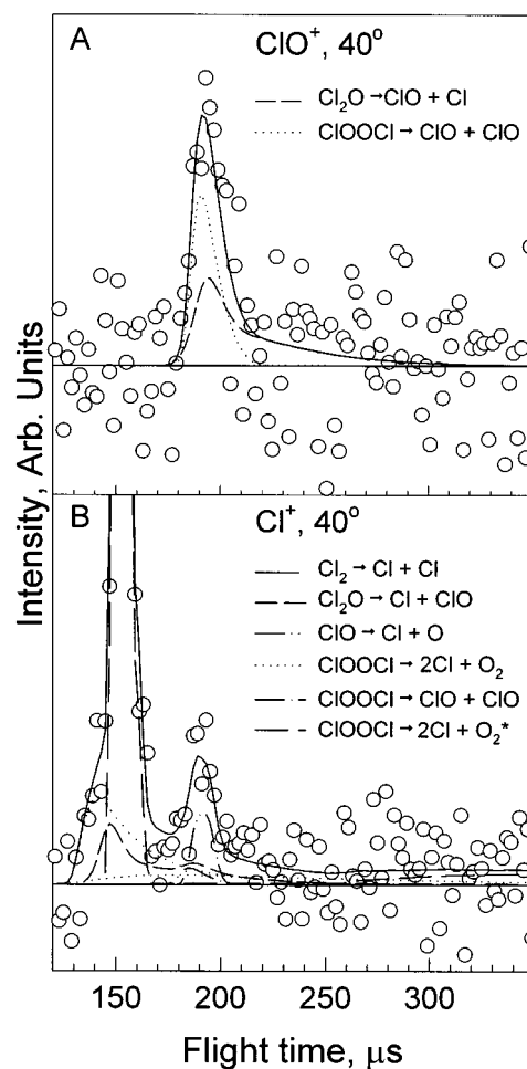
Figure 2. TOF distributions for products from ClOOCl photolysis at 308 nm. TOF spectra were collected at a detector angle of 40° for (A) ClO + and (B) Cl + fragments. The contribution in B from the ClO product channel arises from fragmentation to Cl + in the ionizer.
