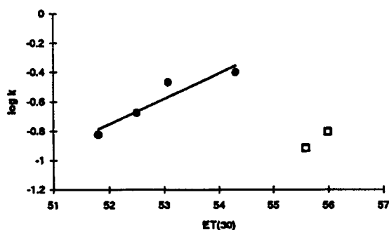
Figure 1. Correlation of reaction rates with E_T(30) values for RuO 4 -mediated oxidations of cis -decalin in (●) acetone–water and (□) acetonitrile–water mixtures
