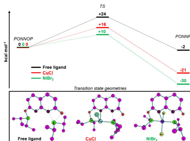
Figure 3. DFT calculated (BP86-D3, def2-TZVP) free energy profiles ( \Delta G^{\circ}_{298K} in kcal mol -1 ) for the rearrangement of PONNOP to PONNP (top) and the transition state geometries (bottom).
