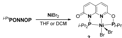
Scheme 4. Synthesis of the mononuclear Ni complex 2 .
