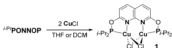
Scheme 3. Synthesis of the dicopper(I) complex 1 .
