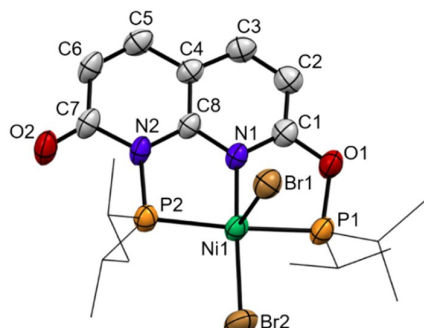
Figure 2. Displacement ellipsoid plot (50% probability) of complex 2 in the crystal. Hydrogen atoms and THF solvent molecules are omitted, and i -Pr groups on P are depicted as wireframe for clarity.
