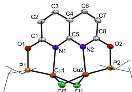
Figure 1. Displacement ellipsoid plot (50% probability) of complex 1 in the crystal. Hydrogen atoms and THF solvent molecule are omitted, and i -Pr groups on P are depicted as wireframe for clarity.
