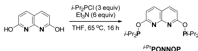
Scheme 2. The synthesis of the i -PrP 2 ONNOP "expanded pincer" ligand.
