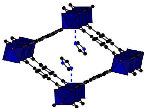
Figure 6: Crystal structure of Al-MIL-53_HIm with some of the imidazole molecules binding to the host framework (view along the channels). AlO 6 polyhedra are shown in dark blue, carbon atoms in black and nitrogen atoms in light blue. The potential hydrogen bonds between the \mu -OH groups and the guest molecules in Al-MIL-53_HIm are shown as dashed blue lines. Please note that most guest molecules adsorbed in Al-MIL-53 (not shown here) assemble in a "random" fashion which we interpret as non-ordered adsorption.
