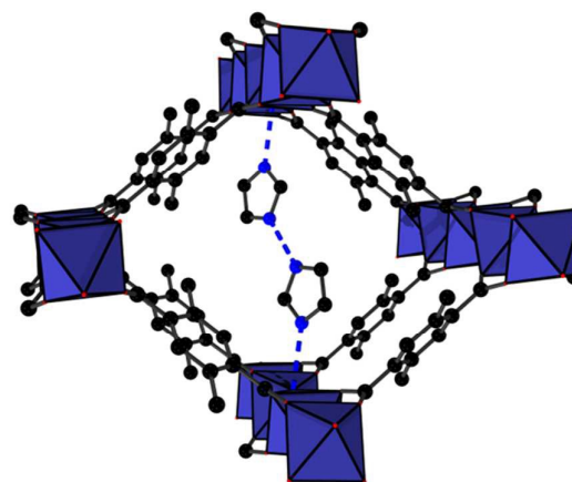
Figure 5: The crystal structure of Al-MIL-53-(CH 3 ) 2 _HIm. AlO 6 polyhedra are shown in dark blue, carbon atoms in black and nitrogen atoms in light blue. The potential hydrogen bonds are shown as dashed blue lines.
