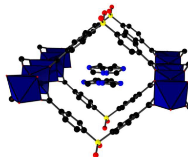
Figure 7: Crystal structure of CAU-11_HIm with some of the imidazole molecules (view along the channels). AlO 6 polyhedra are shown in dark blue, carbon atoms in black and nitrogen atoms in light blue. Please note that all guest molecules adsorbed in CAU-11 assemble in a "random" fashion which we interpret as non-ordered adsorption.
