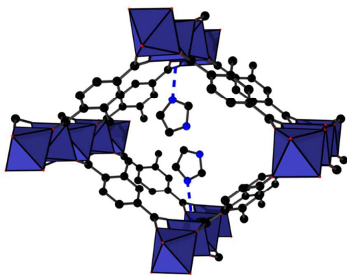
Figure 4: The crystal structure of Al-MIL-53-CH 3 _HIm. AlO 6 polyhedra are shown in dark blue, carbon atoms in black and nitrogen atoms in light blue. The potential hydrogen bonds between the \mu -OH groups and the guest molecules are shown as dashed blue lines.
