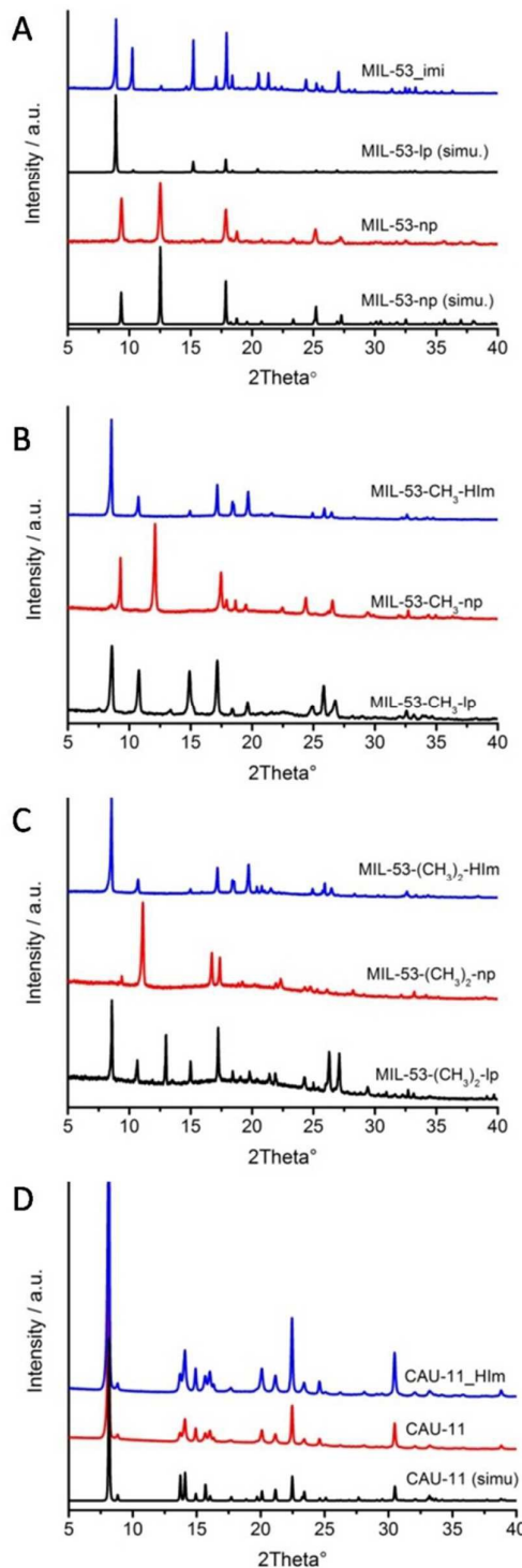
Figure 2: PXRD patterns of: (A) Al-MIL-53 simulated patterns of narrow pore (np) and large pore (lp) form compared to the synthesized compounds; (B) Al-MIL-53-(CH 3 ) and (C) Al-MIL-53-(CH 3 ) 2 experimental patterns of np (narrow pore) and lp (large pore) in comparison with the impregnated compounds. (D) PXRD patterns of CAU-11 simulated, after washing and after impregnation with Him molecules.
