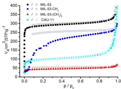
Figure 1: Sorption isotherms of the host materials Al-MIL-53, Al-MIL-53-(CH 3 ), Al-MIL-53-(CH 3 ) 2 and CAU-11.
