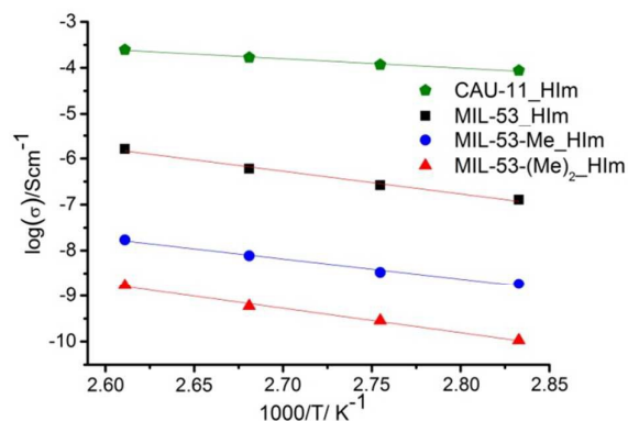
Figure 3: Comparison of the Arrhenius plots of 1 _Hlm (MIL-53_Hlm), 2 _Hlm (MIL-53-CH 3 _Hlm), 3 _Hlm (MIL-53-(CH 3 ) 2 _Hlm) and 4 _Hlm (CAU-11_Hlm). The resulting activation energies are displayed in Table 3.
