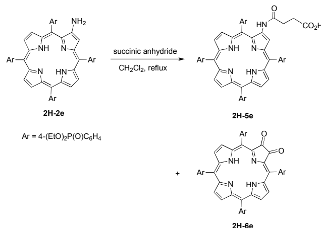
Scheme 3. Acylation of 2-aminoporphyrin 2H-2e .
