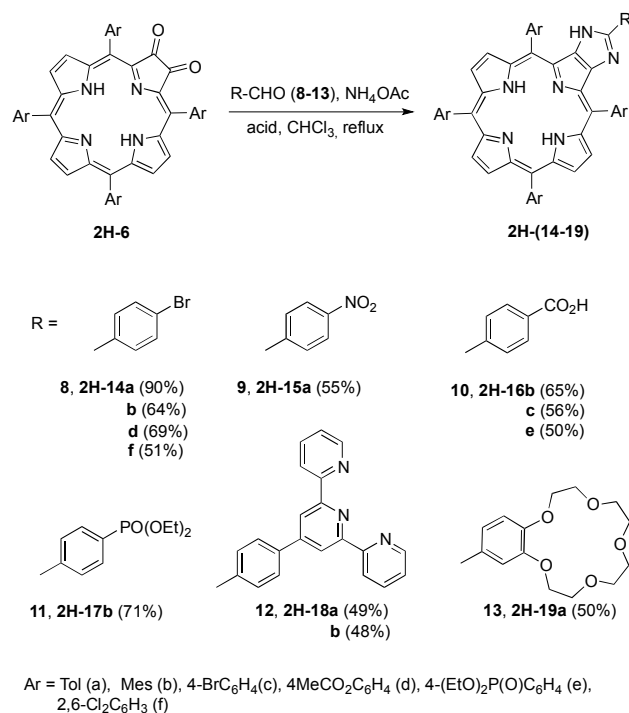
Scheme 5. Synthesis of fused porphyrin imidazole systems through Debus-Radziszewski condensation.
