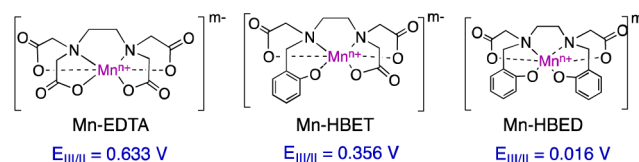
Figure 1. Ligand structure strongly influences the redox potential of the Mn III /Mn II couple. Conversion of carboxylato to phenolato donors shifts the half-cell potential by 617 mV in favor of the higher oxidation state.
