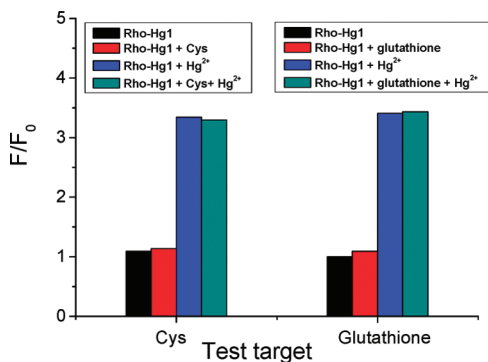
Figure 4. \text{Hg}^{2+} (2 \mu\text{M} ) detection in the presence of L-cysteine and glutathione (100 \mu\text{M} ) in ethanol/HEPES buffer (1/1, v/v, pH 7.0, 50 mM), [Rho-Hg1] = 0.3 \mu\text{M} . Excitation wavelength is 510 nm.
