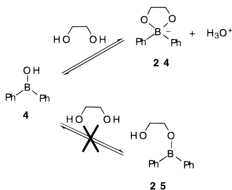
Figure 6. Covalent complexation between a diol and 4 in aqueous solution only producing the chelated tetrahedral boronate anion 24 and not the monodentate trigonal ester 25 .
