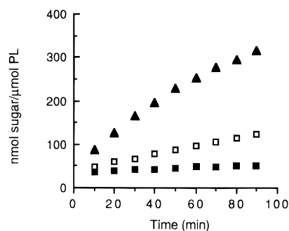
Figure 3. Efflux profiles for liposomes containing 300 mM of ▲ sorbitol, □ fructose, or ■ glucose after treatment with phenylboronic acid ( 1 , 1 mM) at pH 7.5. Liposome composition DPPC:C:PA, 20:15:2; total lipid concentration 0.75 mM, T = 25^\circ\text{C} , PL = phospholipid, reproducibility \pm 10\% .
