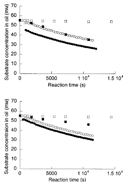
Figure 8. Top: Effect of a catalytical amount of TBAHS on the reaction between 4-TBBB and KI at 23°C in D_2O/C_8G_1/CH_2Cl_2 (○, ●) and D_2O-CH_2Cl_2 (□, ■). Bottom: Effect of a catalytical amount of [18]crown-6 on the reaction between 4-TBBB and KI at 23°C in D_2O/C_8G_1/CH_2Cl_2 (○, ●) and D_2O-CH_2Cl_2 (□, ■). In both graphs open symbols denote reaction without PTA and black symbols reactions with PTA. The overall concentrations of both 4-TBBB and KI are 20mM, and of PTA 0.2mM.
