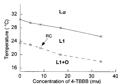
Figure 1. Phase diagram of the ternary D 2 O/C 12 E 5 /decane system in presence of 4-TBBB. The weight ratio between oil and surfactant is 48/52 and the total weight fraction of oil + surfactant is 0.2. Raising the temperature gives a transition from an oil-in-water microemulsion in equilibrium with excess oil (L1+O phase) to an oil-in-water microemulsion (L1 phase) and on to a lamellar liquid crystalline phase (L α phase). The arrow indicates the reaction composition (RC).
