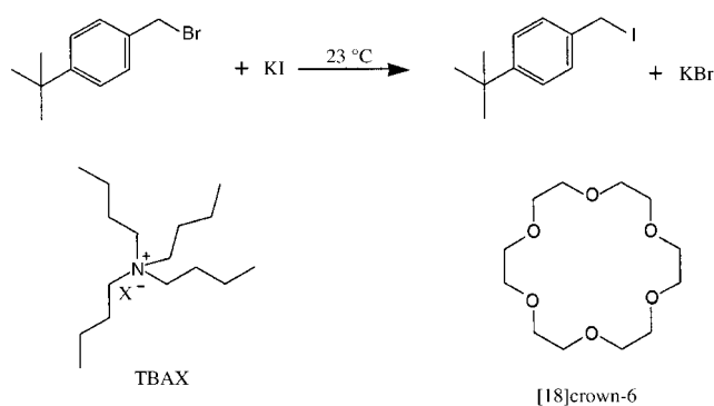
Scheme 1. Top: Nucleophilic substitution reaction between 4-TBBB and KI. Bottom: Structures of TBAB (X=Br), TBAHS (X=HSO 4 ) and [18]crown-6.
