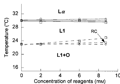
Figure 2. Phase diagram of the ternary D 2 O/C 12 E 5 /decane system in presence of KI (○), TBAHS (□) and [18]crown-6 (◇). The weight ratio between oil and surfactant is 48/52 and the total weight fraction of oil + surfactant is 0.2. Raising the temperature gives a transition from an oil-in-water microemulsion in equilibrium with excess oil (L1+O phase) to an oil-in-water microemulsion (L1 phase) and on to a lamellar liquid crystalline phase (L α phase). The arrow indicates the reaction composition (RC). Addition of the second reactant, 4-TBBB induces a downward slope of both the upper and the lower phase boundary curves (see Figure 1). Thus, the reaction composition lies within the one-phase region in all cases.
